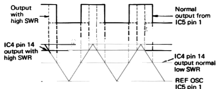
Fig. 11 Automatic SWR computing circuit waveforms
