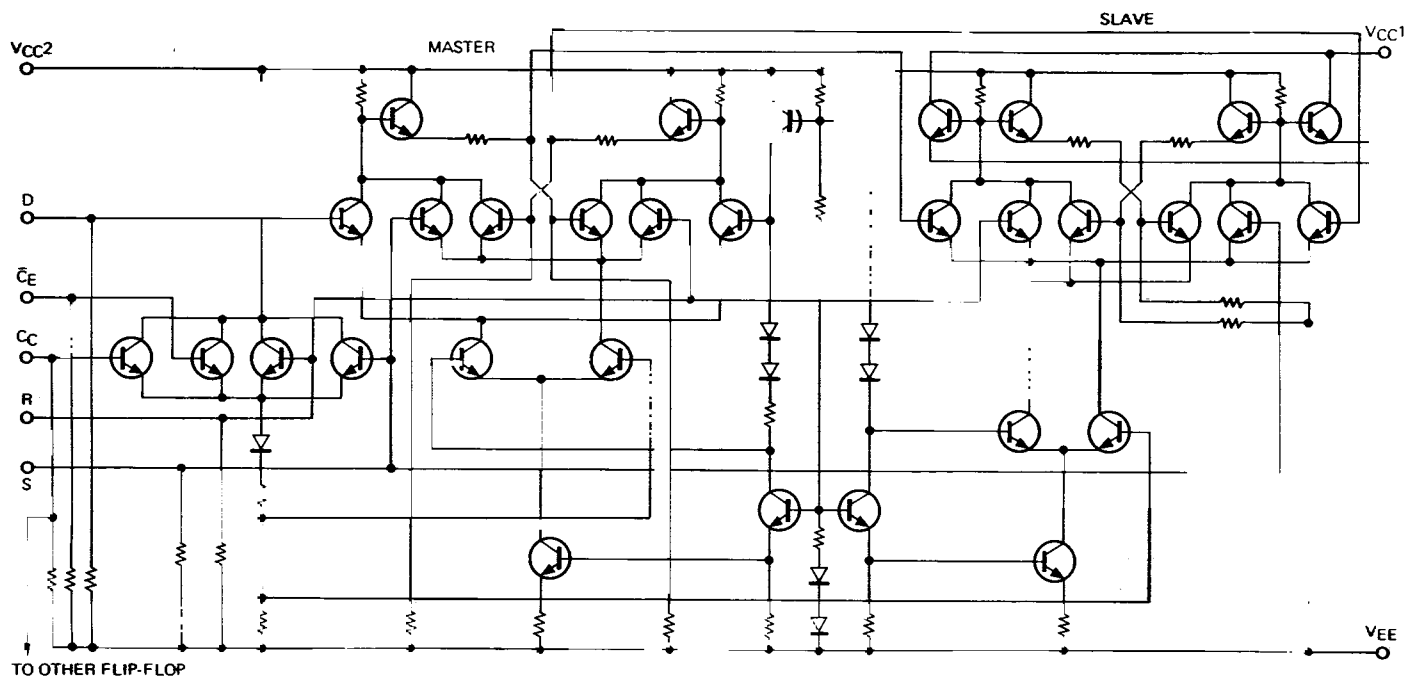
HD10131 Equivalent circuit 1/2 (AT unit Q29)
