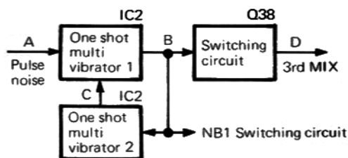
Fig. 7 NB2 circuit
