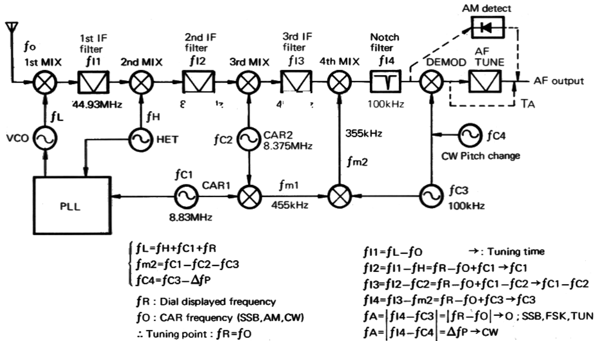
Fig. 12-A RX configuration Normal (wide) response
